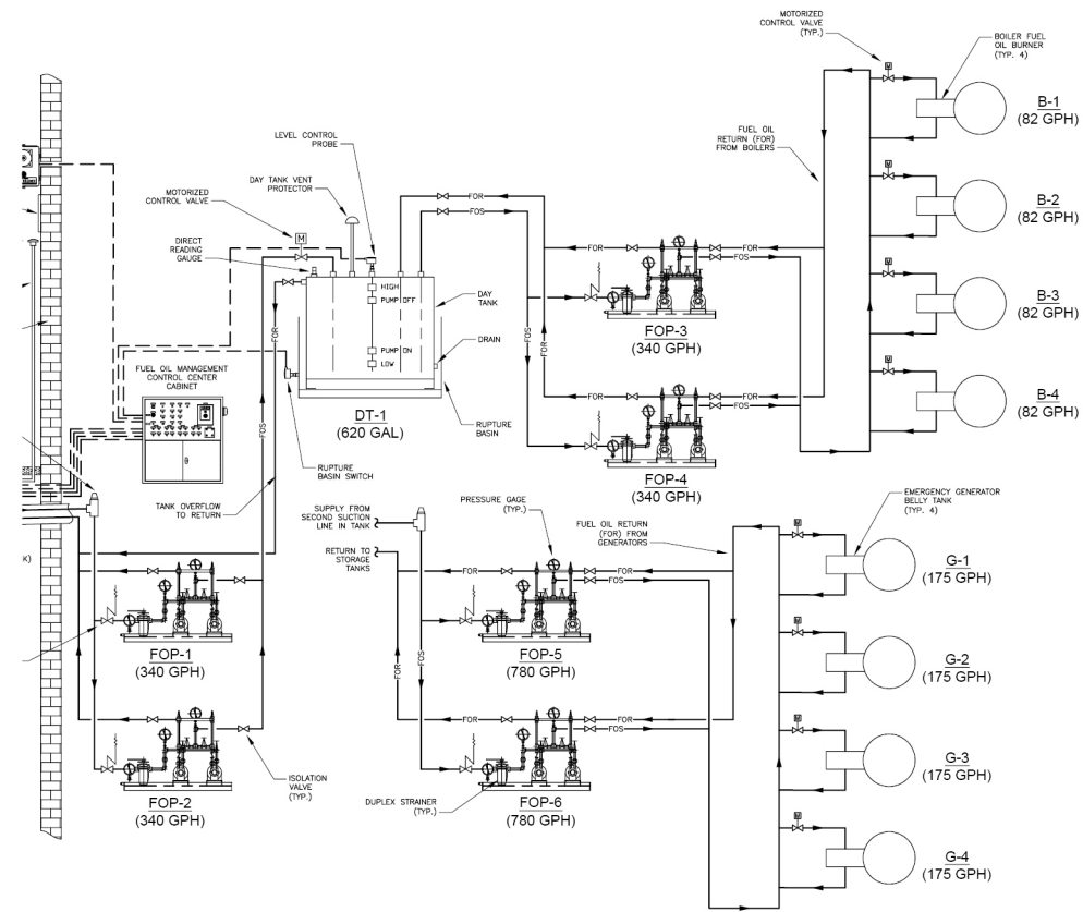
FUEL OIL FLOW DIAGRAM - PART B
